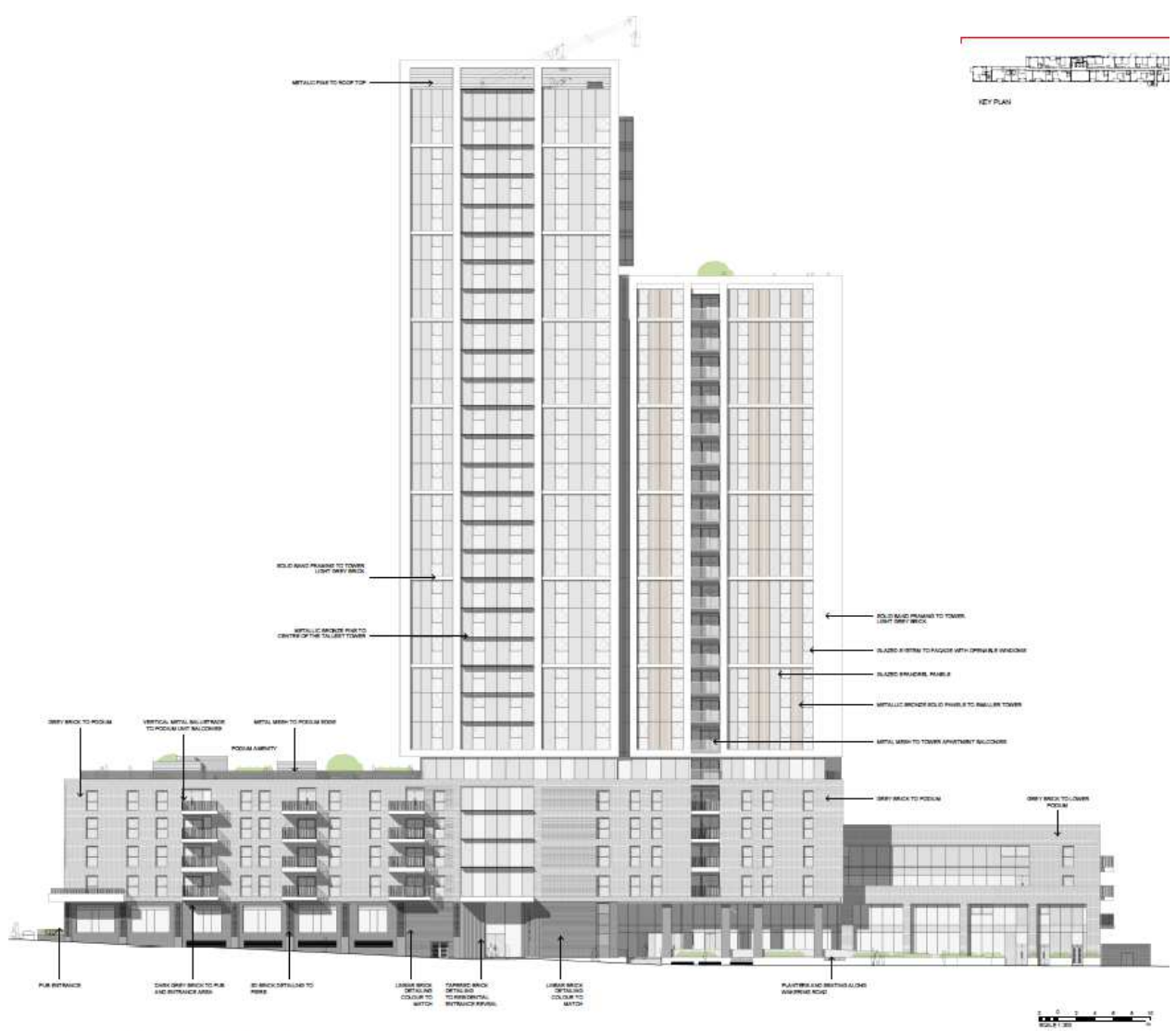
PROPOSED NORTH EAST ELEVATION 1:200
