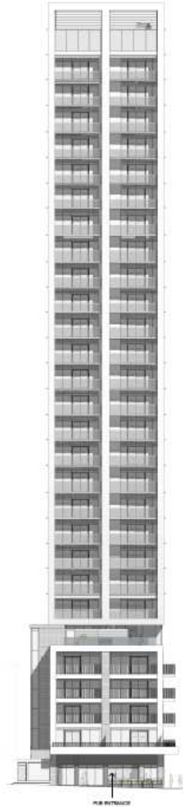
② PROPOSED SOUTH EAST ELEVATION 1:200
