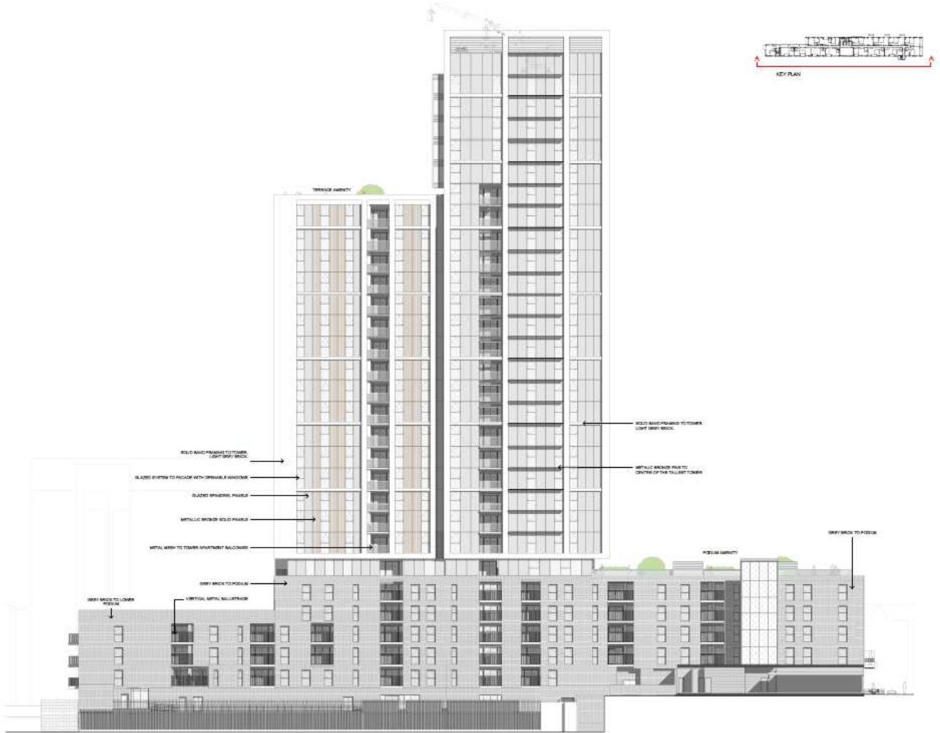
① PROPOSED SOUTH WEST ELEVATION 1:200
