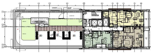
1 PROPOSED 22ND FLOOR PLAN 1:100
